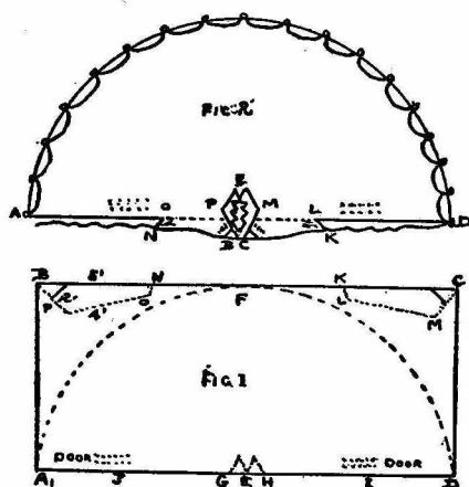
THE TEN FOOT TEEPEE
