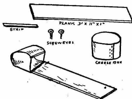
HOME MADE TOBOGGAN.
