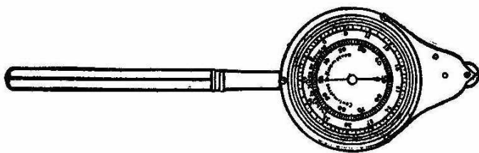
Universal Map Measure,
